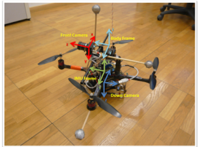
Fig. 1. Quadrotor frames [18]
